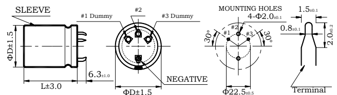
Φ 35 O-Type P-Type: With short pin (4±1) Lock Terminal Unit:mm
